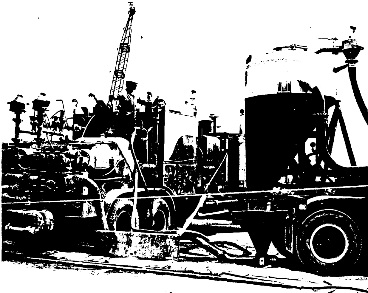
Figure 6-20. Standard twin HT-400 cementing unit fully rigged with jet mixing cone and slurry reservoir. Courtesy, Halliburton Services
