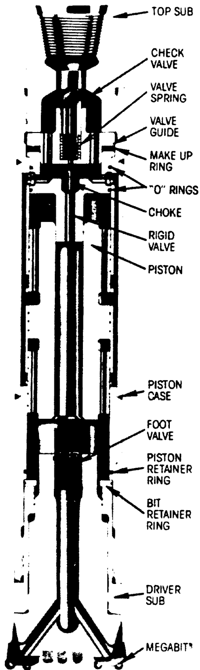
Figure 6-5. Down-hole hammer
