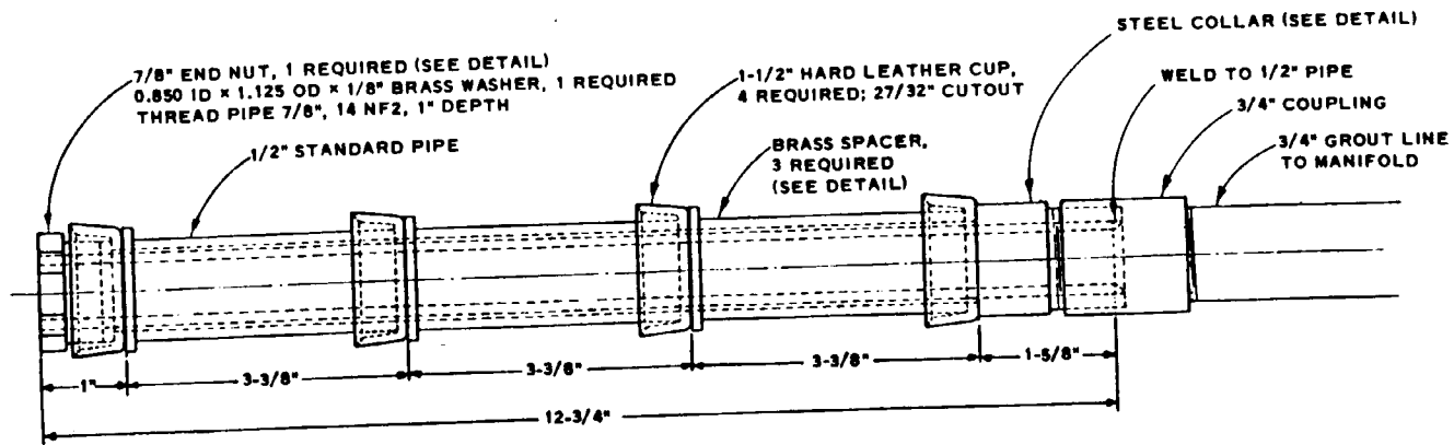
PACKER ASSEMBLY
