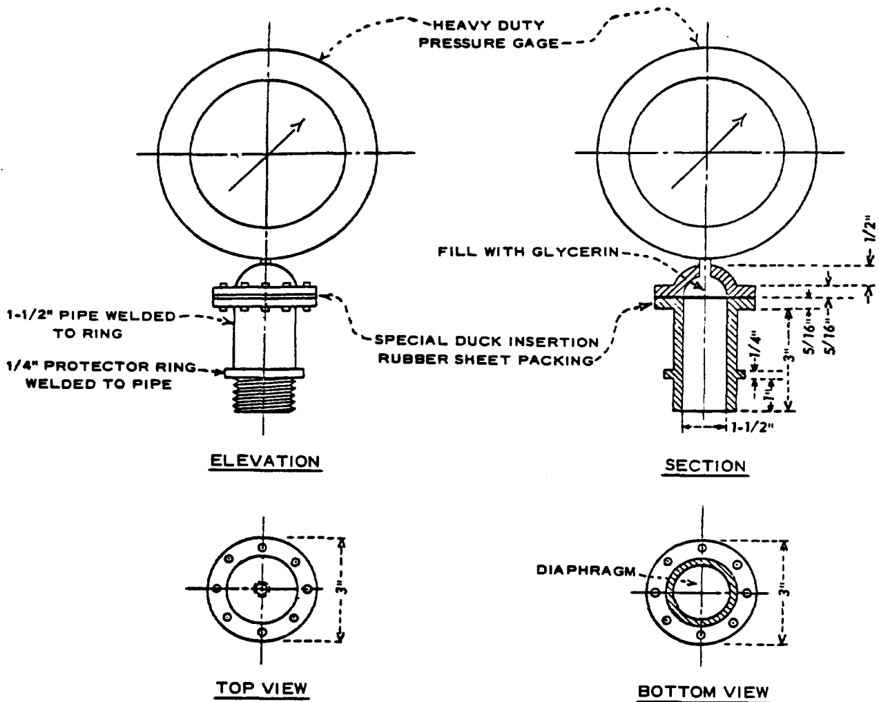
Figure 6-22. Glycerin-filled gage saver
