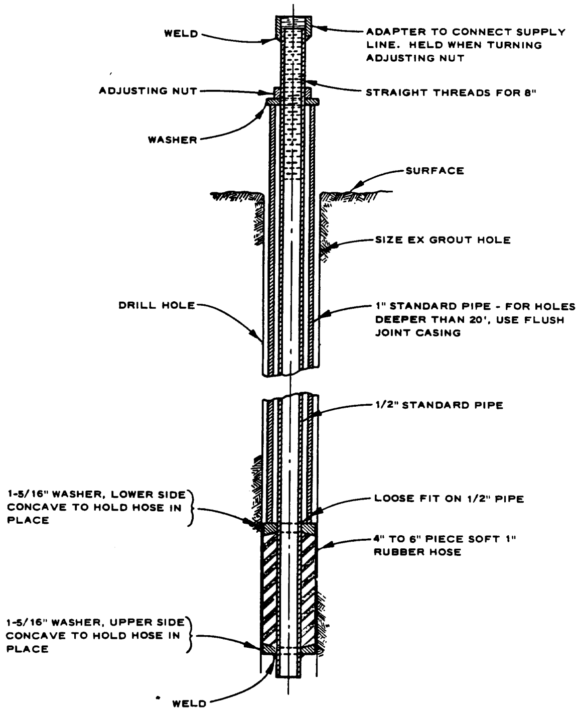
Figure 6-16. Mechanical packer
