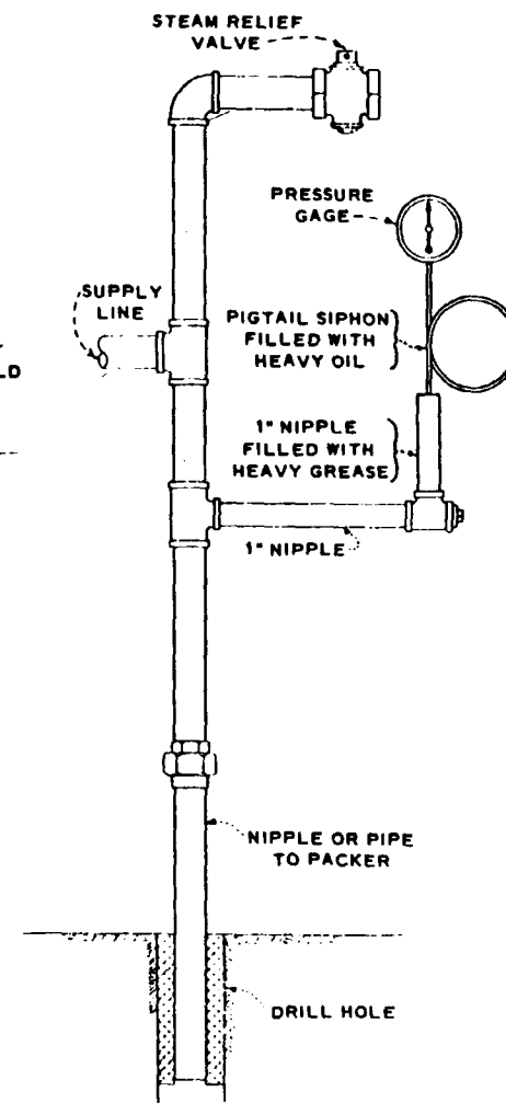
TYPICAL ASPHALT GROUTING MANIFOLD AND CONNECTIONS
