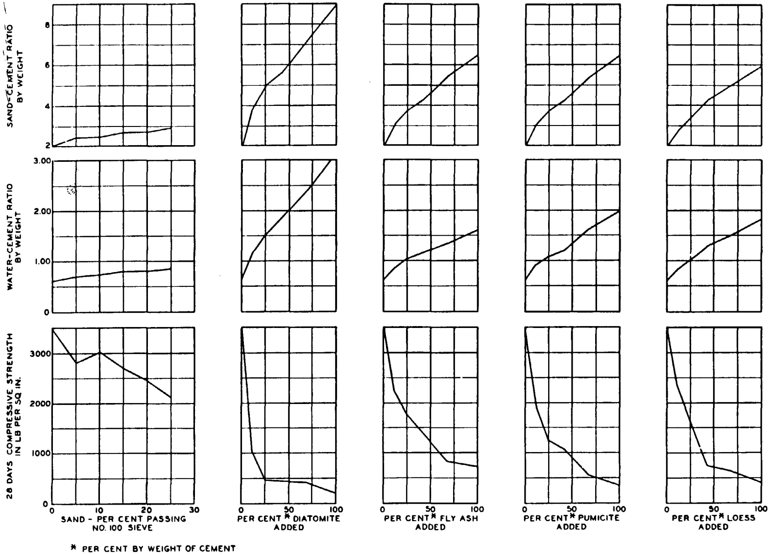
Figure D-1. Characteristics of grout mixtures
