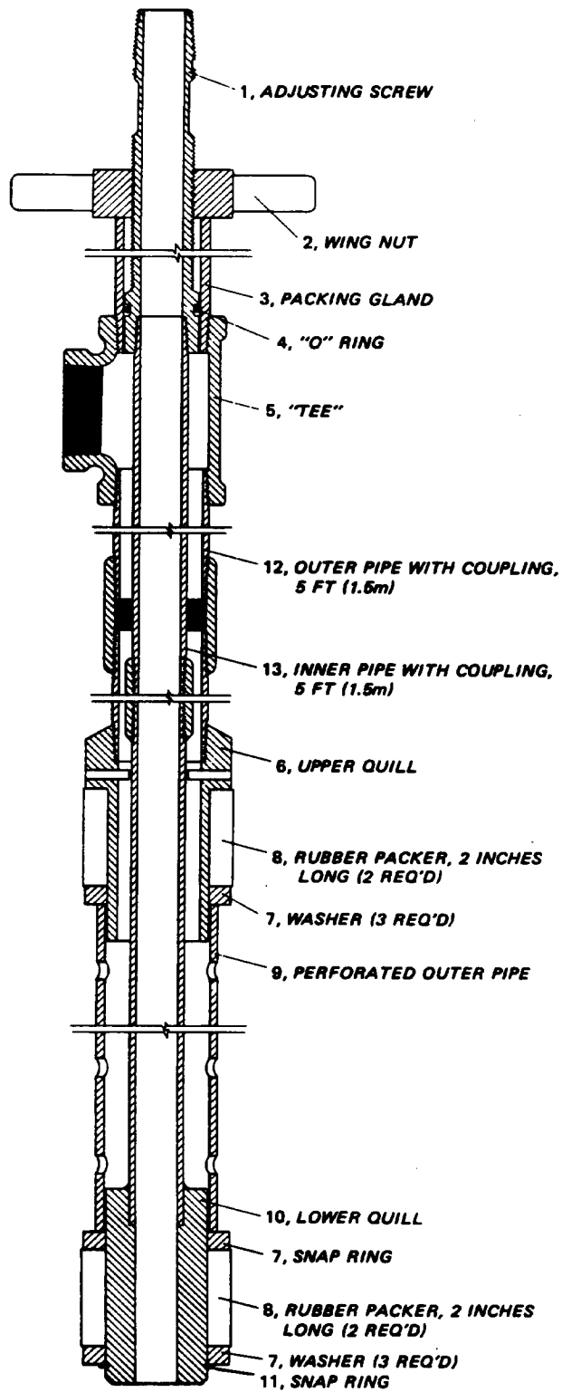
Figure 6-21. Pressure testing packer assembly
