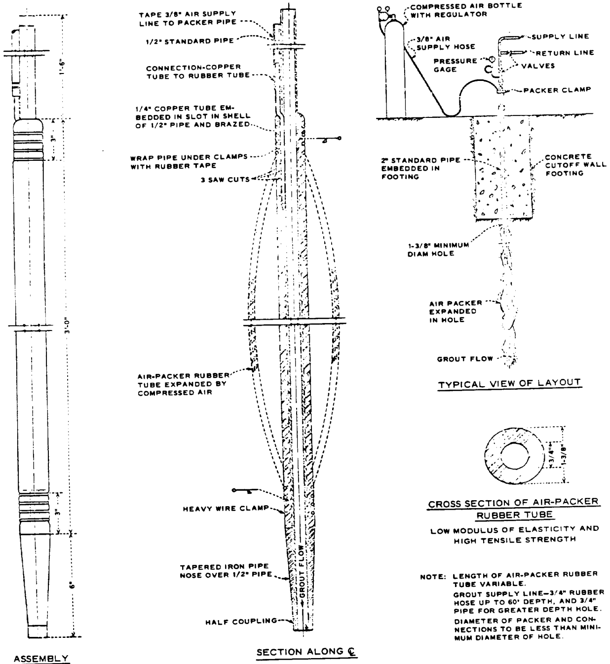
Figure 6-17. Air packer
