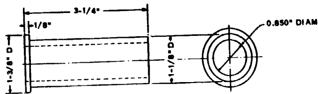
DETAIL OF PACKER SPACER
