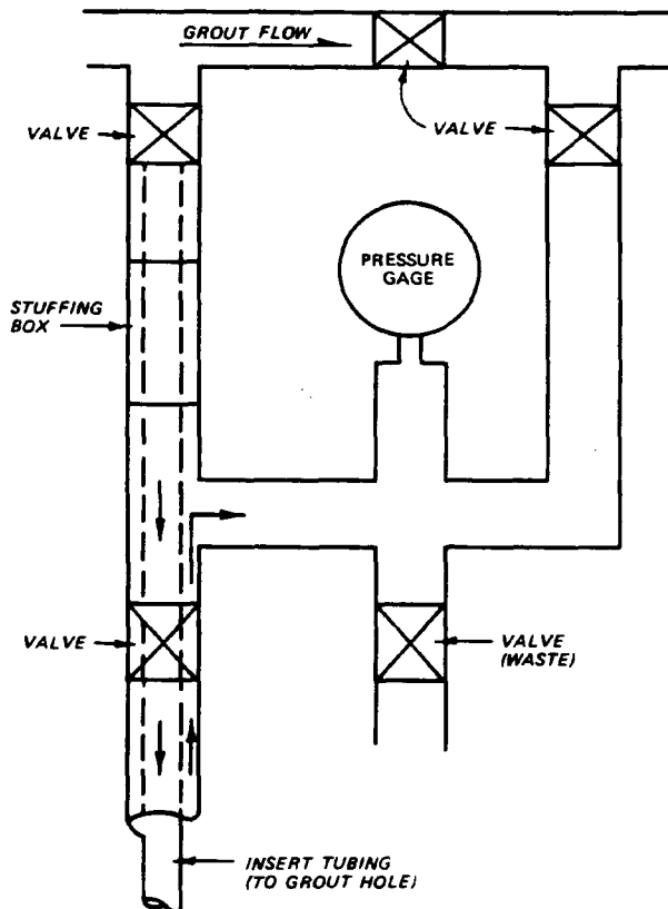
Figure 6-14. Circuit grouting header (not to scale)
