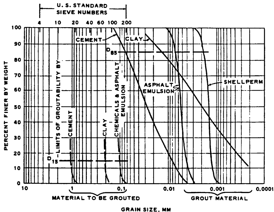
Figure 5.1 Soil and grout materials grain-size curves
