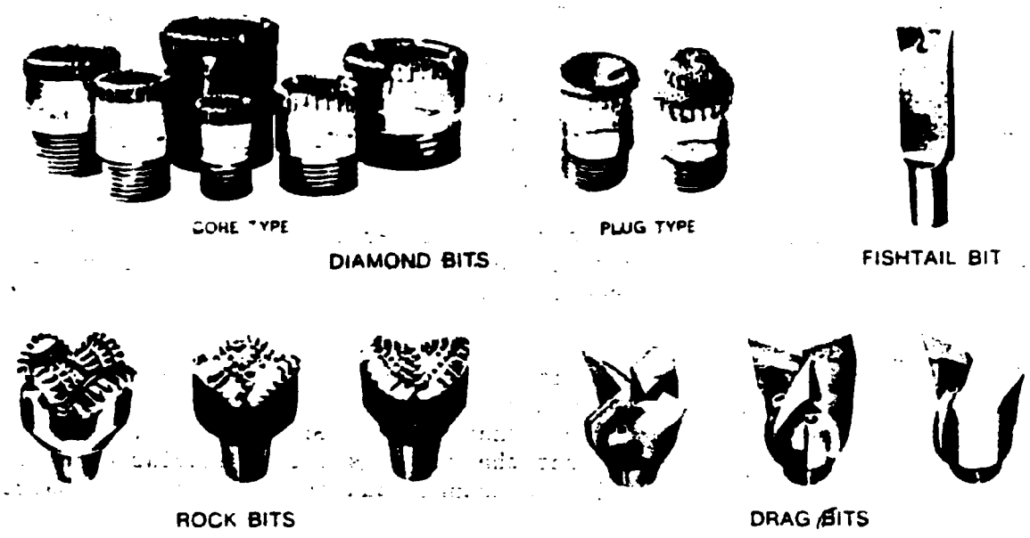
Figure 6-6. Drill bits
