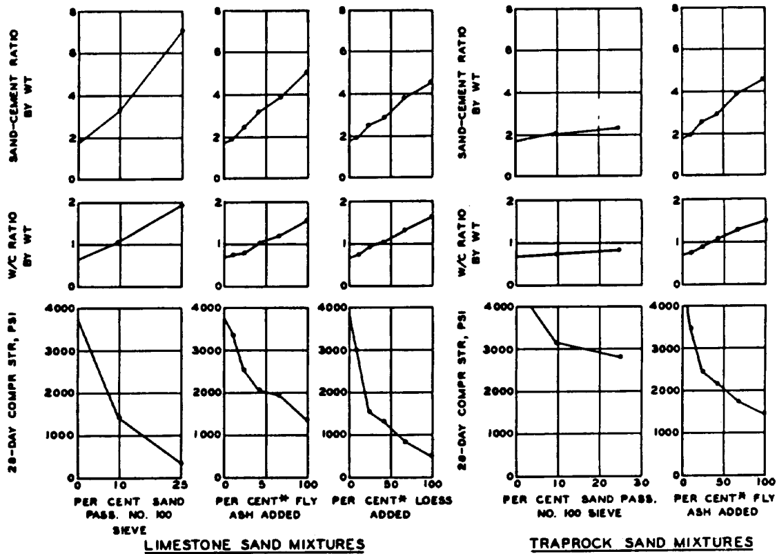
Figure D-2. Compressive strength, water-cement, and sand-cement ratios of the grout mixtures
