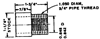
DETAIL OF COLLAR
