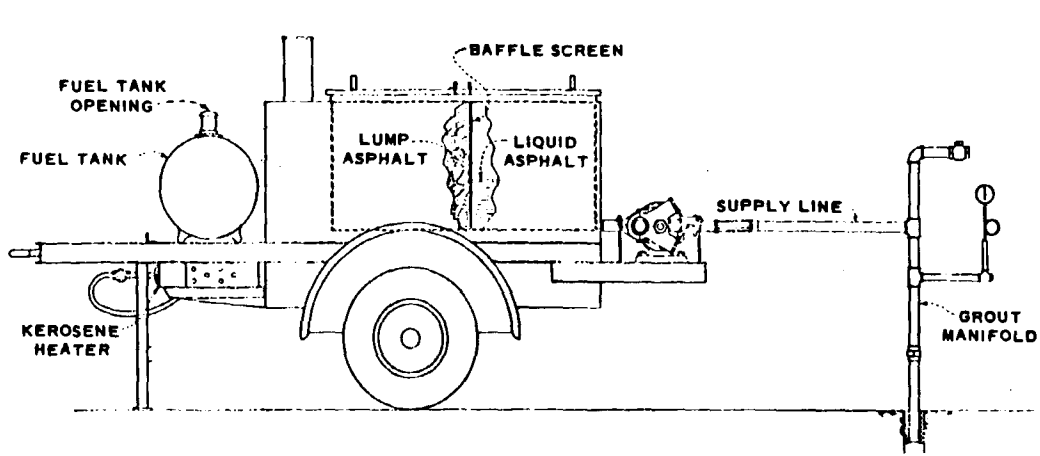
ASPHALT HEATER WITH GROUT CONNECTIONS
