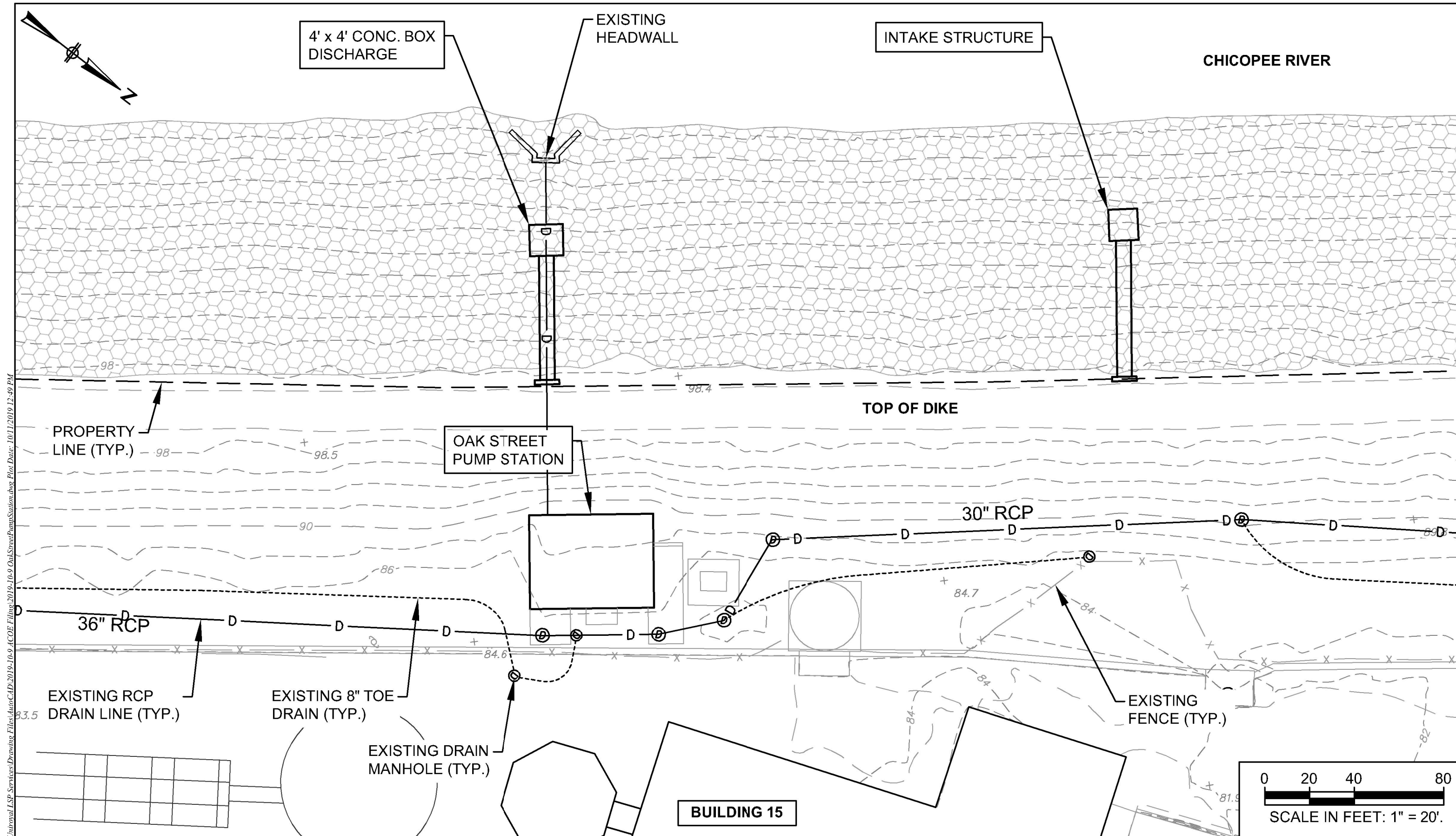
Figure No. 7 Oak Street Pump Station & Intake Tunnel Plan
