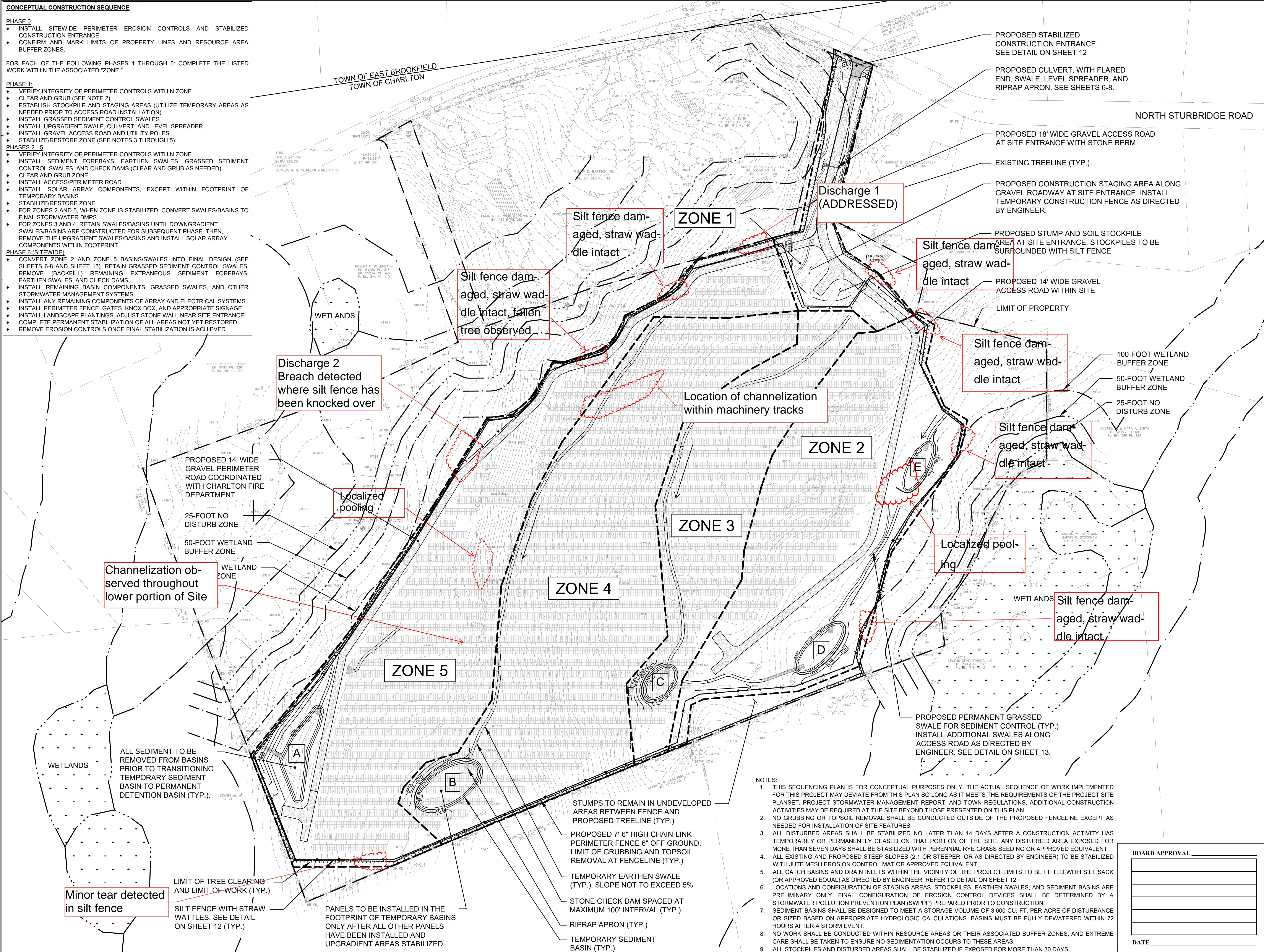
FIGURE 1: SWPPP INSPECTION SKETCH 10/29/2021
