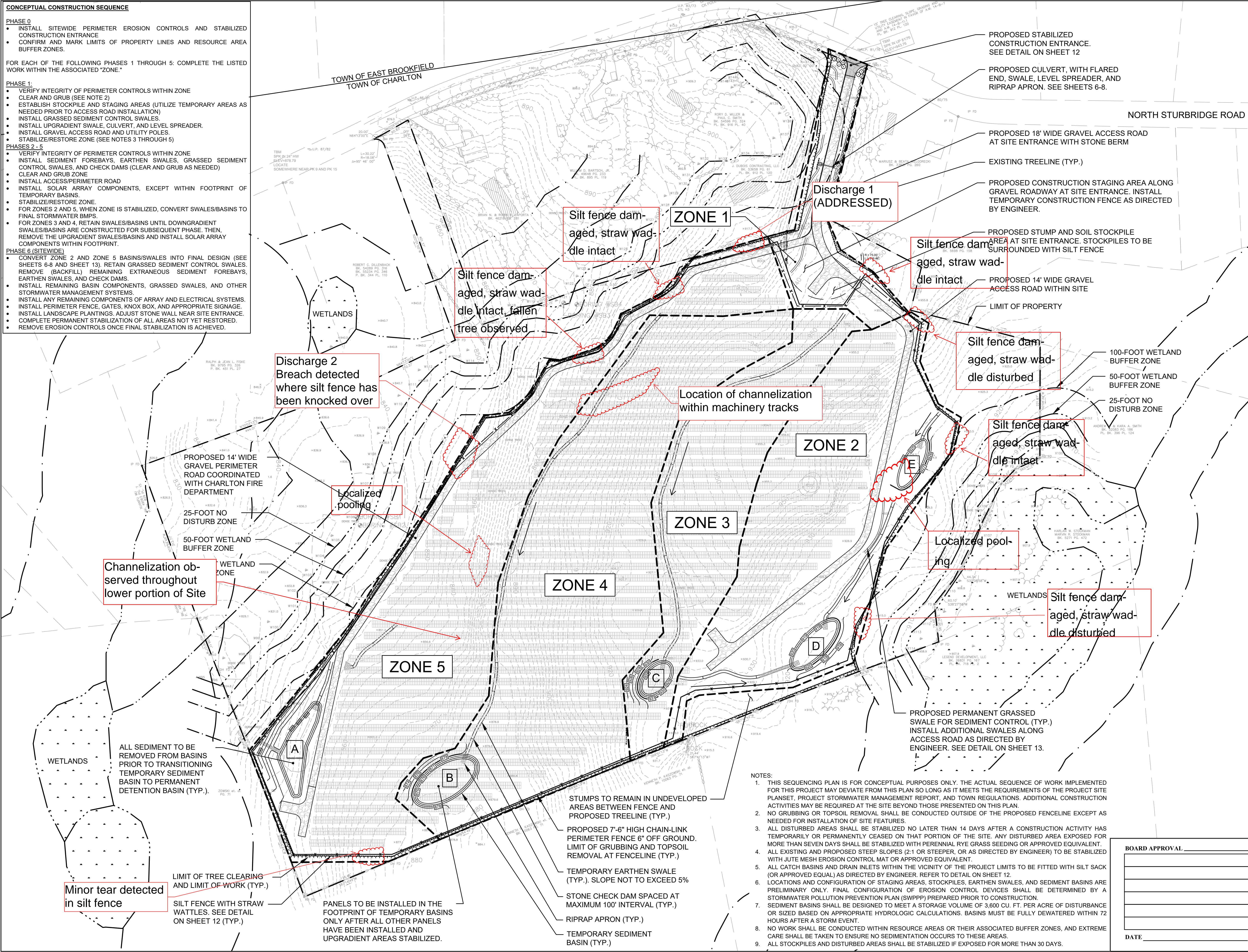
FIGURE 1: SWPPP INSPECTION SKETCH 12/27/2021
