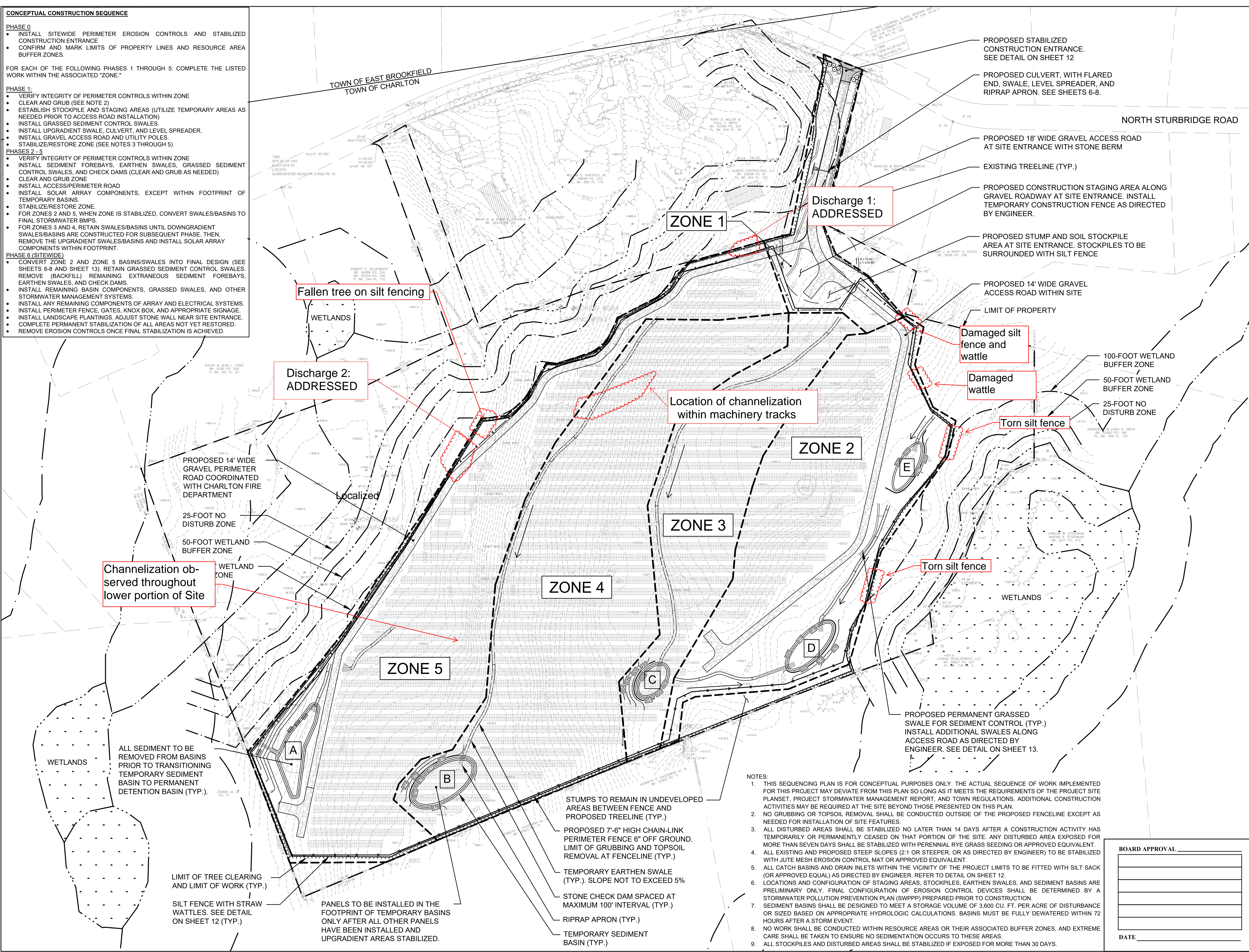
FIGURE 1: SWPPP INSPECTION SKETCH 7/14/2022
