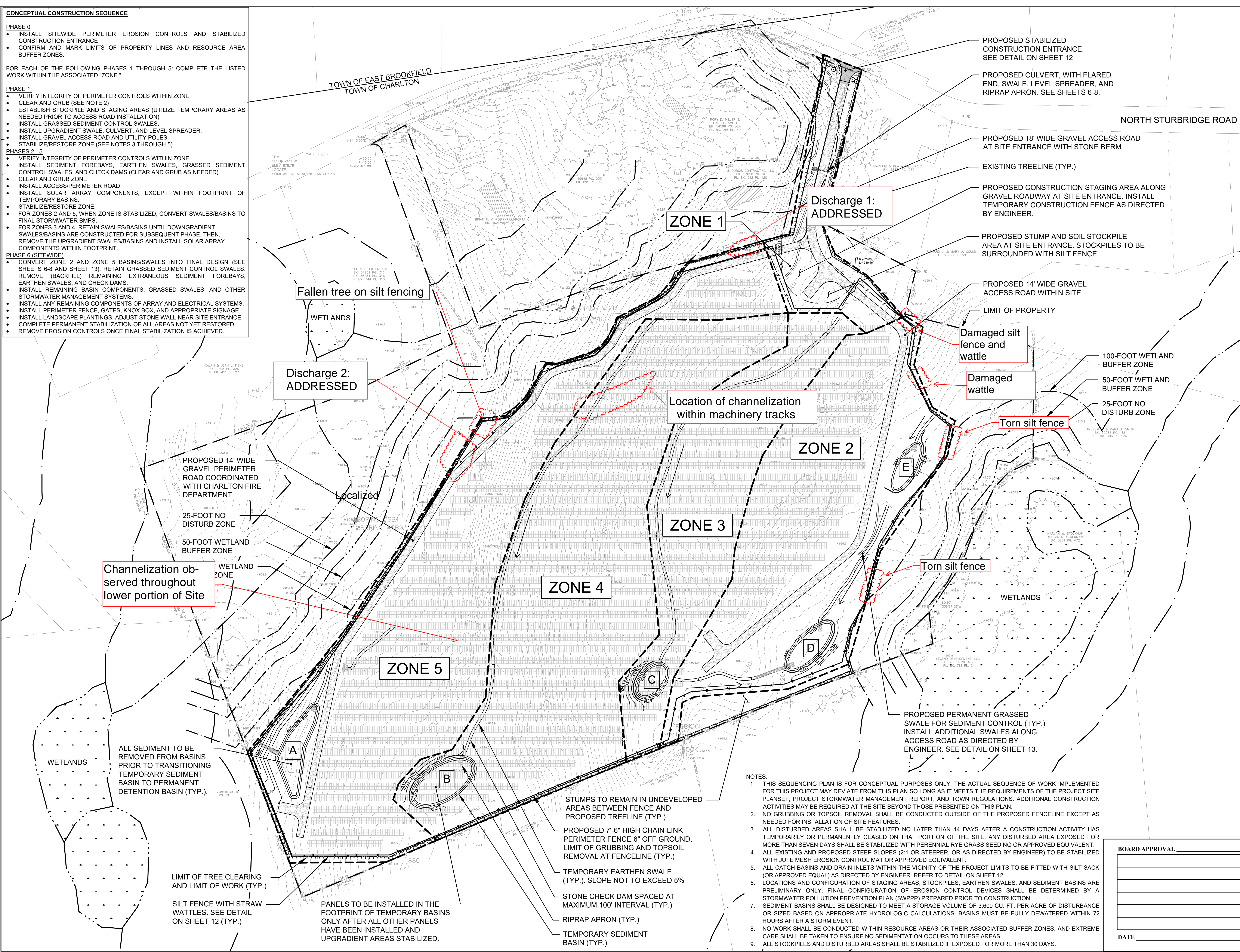
FIGURE 1: SWPPP INSPECTION SKETCH 7/19/2022
