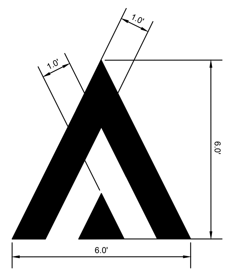
PAVEMENT MARKING DETAIL NOT TO SCALE
