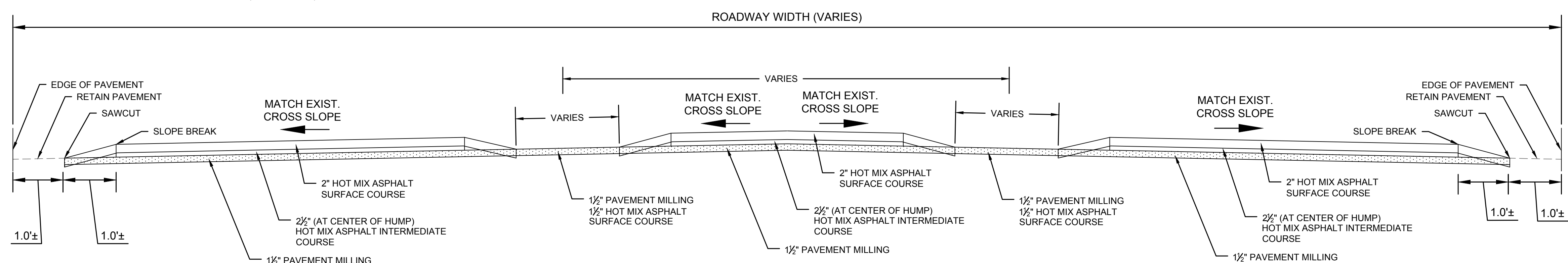
SECTION B-B NOT TO SCALE
