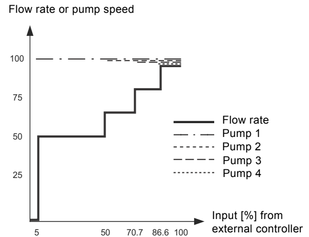
Fig. 34 Regulation curve for MPC-S system in open loop
