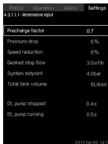
Fig. 77 Alternative input
