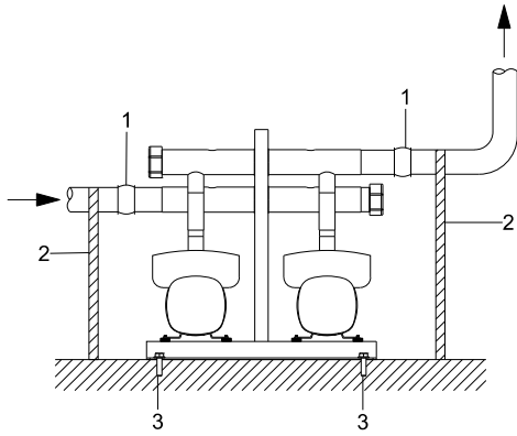
Fig. 2 Example showing the position of expansion joints, pipe supports and mounting bolts
