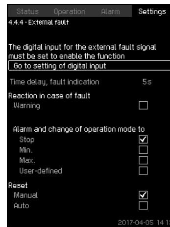
Fig. 113 External fault
