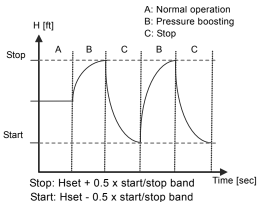
Fig. 74 On/off operation
