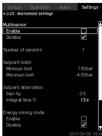
Fig. 104 Multisensor settings
