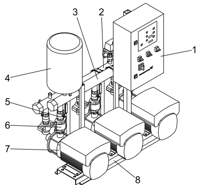
Fig. 8 Front view of Hydro MPC CME pump system with three CM(E) pumps
