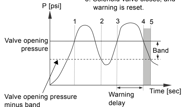
Fig. 117 Pressure relief
