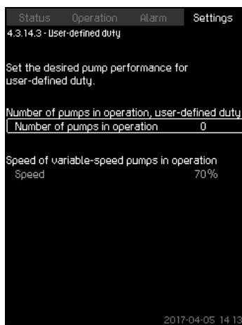
Fig. 94 User-defined duty
