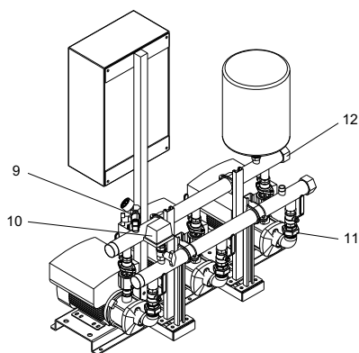
Fig. 9 Rear view of Hydro MPC CME pump system with three CM(E) pumps
