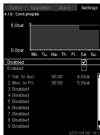
Fig. 53 Clock program
