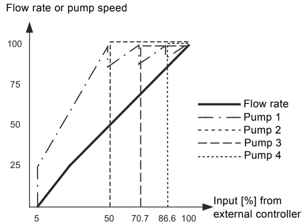
Fig. 33 Regulation curve for MPC-F system in open loop
