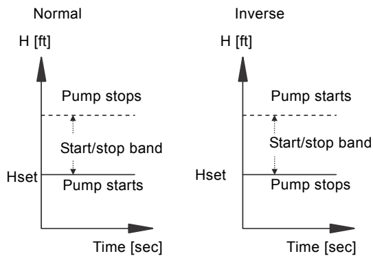
Fig. 58 Normal and inverse control
