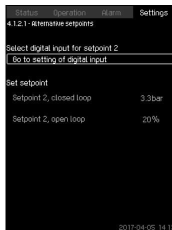
Fig. 47 Alternative setpoints 2-7
