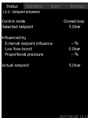
Fig. 19 Setpoint influence
