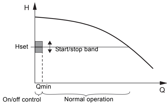
Fig. 73 Start/stop band
