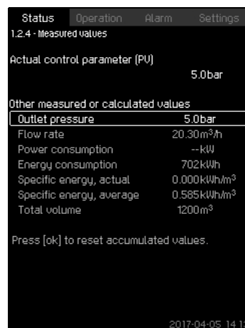
Fig. 20 Measured values
