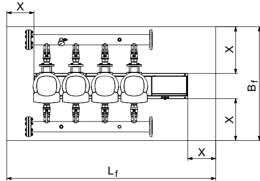
Fig. 3 Foundation
