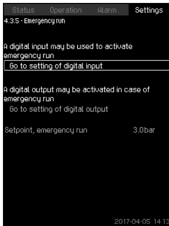
Fig. 80 Emergency run
