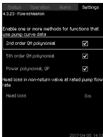
Fig. 102 Flow estimation
